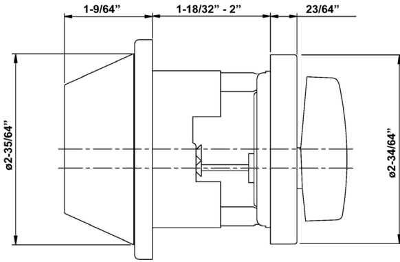
220-Series, IC Core
