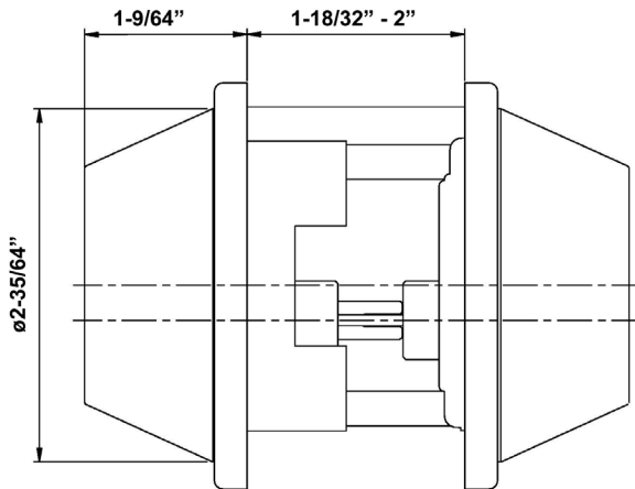
225-Series, IC Core
